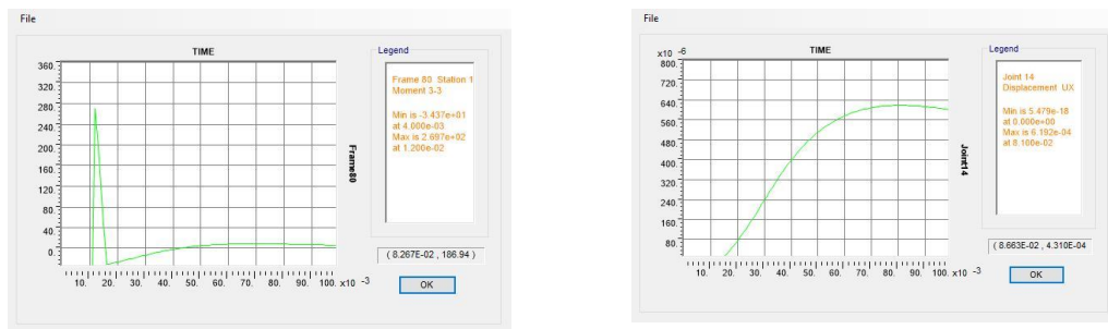
Figure 7 Moment and Displacement Time History of Selected Column removed
