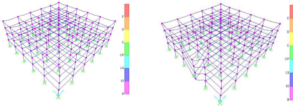
Figure 6 Hinges and deformed shape for blast analysis (60kg Charge)
