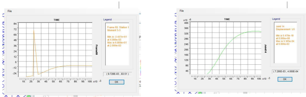
Figure 5 Moment and Displacement Time History of Selected Column removed
