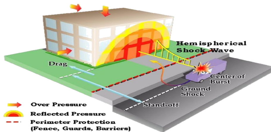
Figure 1 Blast Pressure Propagation Parameters (FEMA-427 2003) [9]
