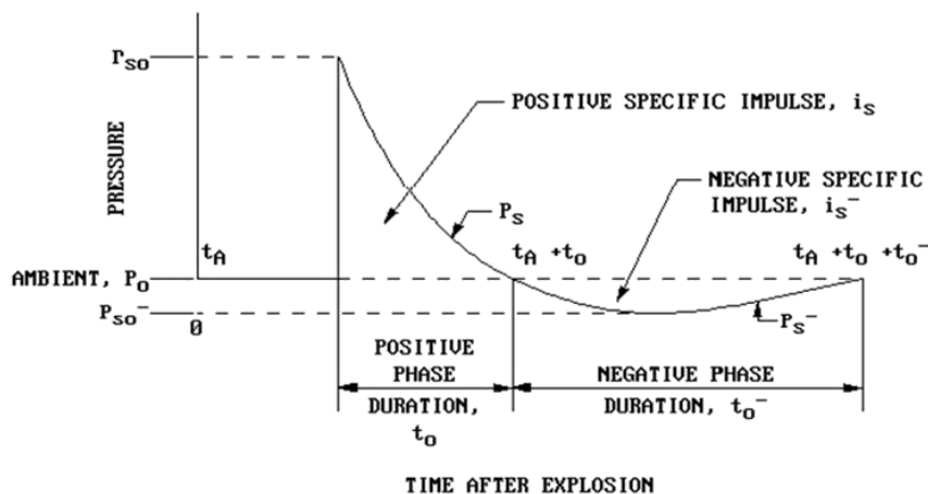
Figure 2 Free-Field Pressure-Time Variation (UFC 3-340-02 2014) [7]
