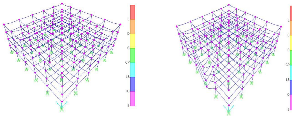
Figure 4 Hinges and deformed shape for blast analysis (30kg Charge)
