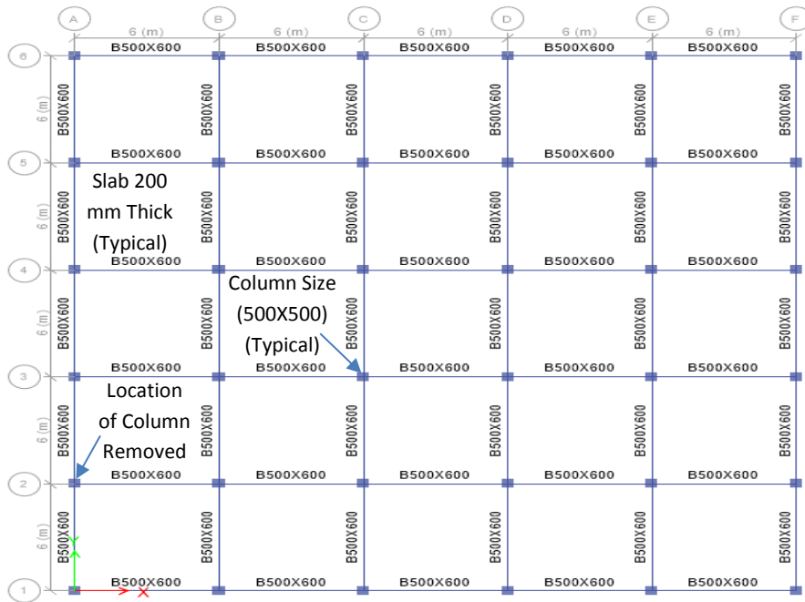
Figure 3 Reinforced Concrete Building Plan and Location of Column Removed
